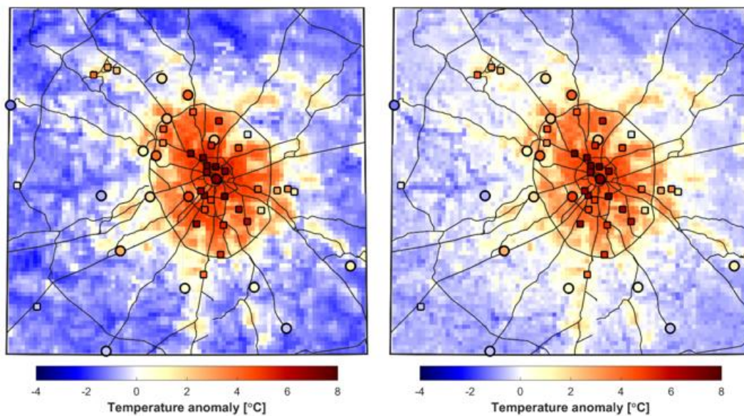
Figure 14: The spatial structure of the average nocturnal (00UTC) urban temperature anomaly in Moscow region according to observations (coloured squares and circles) and simulations v5_MOD (left) and v505_REF (right), shown as coloured background. The averaging is performed over 20-27 May 2014. The temperature anomaly is defined as a deviation from the mean rural value, averaged over 9 rural reference weather stations.
