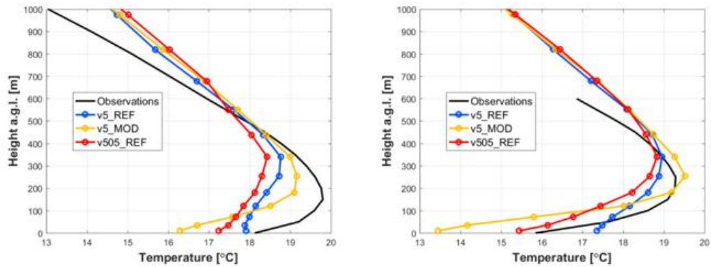
Figure 13: The observed and simulated nocturnal (00UTC) vertical temperature profiles, averaged over the period of 20-27 May 2014 for CAO suburb site (left) and Zvenigorod rural site(right).
