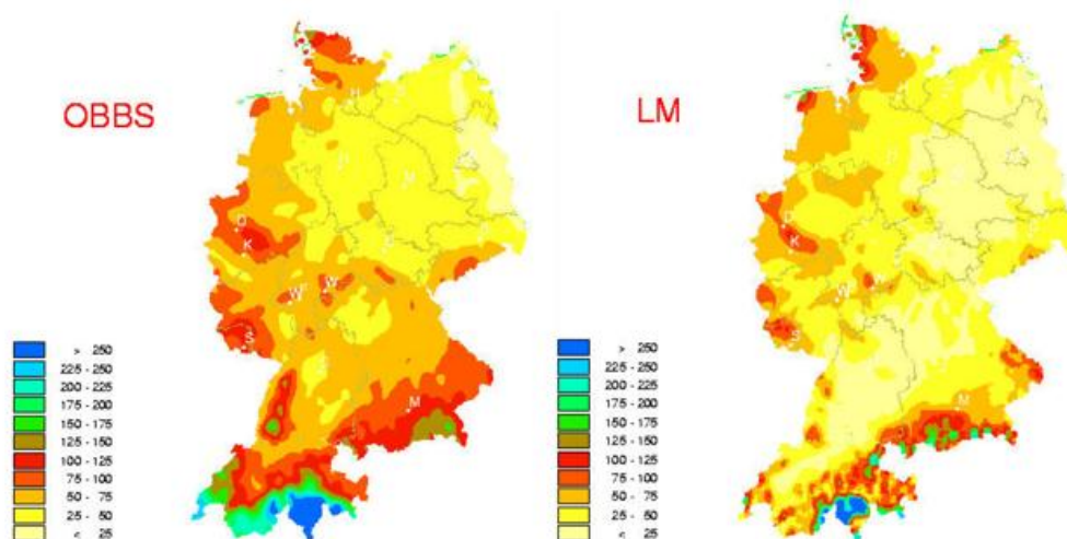
Figure 8: Monthly precipitation amount (mm) for October 2000 as observed (OBBS) by climate networks (max: 525 mm, mean: 63mm) and derived from 00 UTC LM forecasts (+30h - 06h) at DWD (max: 999 mm, mean: 69mm).
