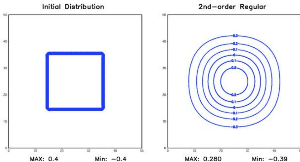
Figure 4: Contour maps of a field for the 2D square wave test. Left: Initial field distribution, where a block with field values with 0.4 is placed in a background field having the value of -0.4. Right: Solution of the 2nd-order regular diffusion after 100 time steps. The contour interval is 0.1
