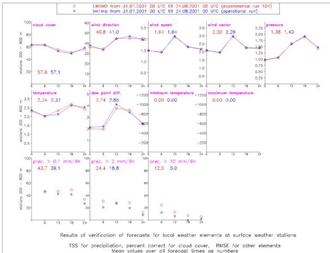
Figure 16: As in Figure 15 except for all Synop Stations with an altitude between 300m and 800m above sea-level.
