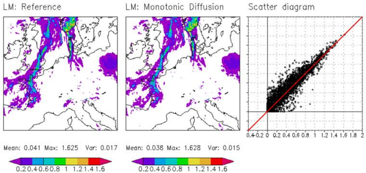
Figure 7: Vertically integrated cloud water ( \text{kg}/\text{m}^2 ) content of a 12-h LM forecast starting at 18 September 2000 00 UTC. Left: reference solution with 4th order regular diffusion; middle solution from a run with monotonic Xue limited diffusion; right: Scatter diagram of values from the reference (y-axis) viz. experiment (x-axis) runs.
