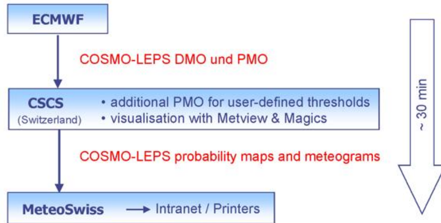
Figure 25: Flow chart of the MeteoSwiss post-processing of COSMO-LEPS output.
