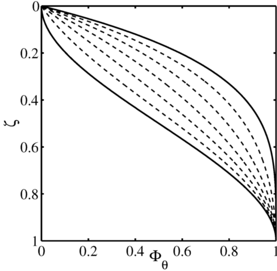
Figure 5: The fourth-order polynomial approximation of the shape function \Phi_\theta(\zeta) with respect to the temperature profile in the thermocline. The curves are computed from Eq. (55) with seven different values of the shape factor C_\theta ranging from C_\theta = C_\theta^{min} = 0.5 , lower solid curve, to C_\theta = C_\theta^{max} = 0.8 , upper solid curve, \Delta C_\theta = 0.05 apart.
