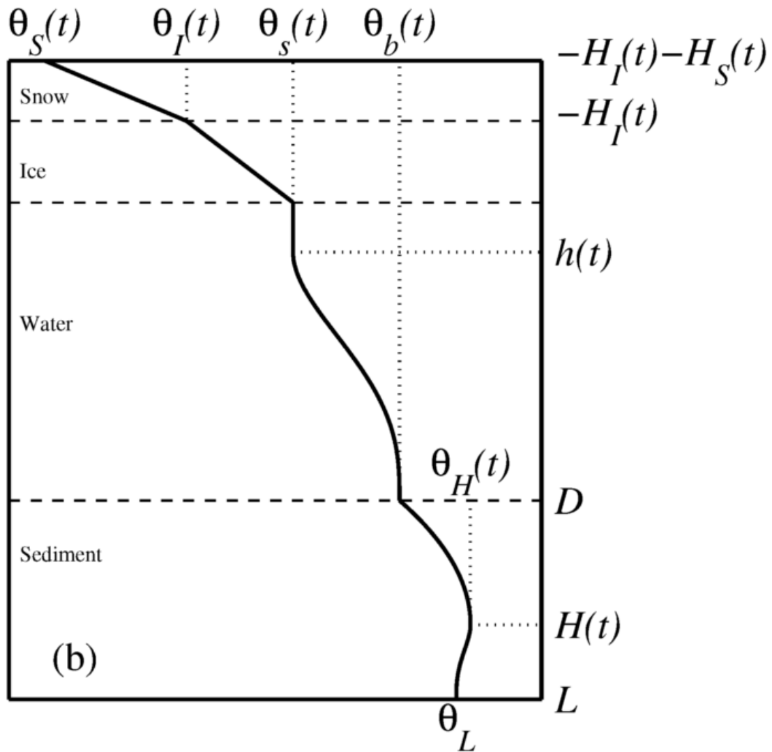
Figure 4: Apart from \theta_s(t) , h(t) , \theta_b(t) , C_\theta(t) , \theta_H(t) , and H(t) (see Fig. 3), four additional quantities are computed in case the lake is covered by ice and snow. These are the temperature \theta_S(t) at the air-snow interface, the temperature \theta_I(t) at the snow-ice interface, the snow depth H_S(t) , and the ice depth H_I(t) .
