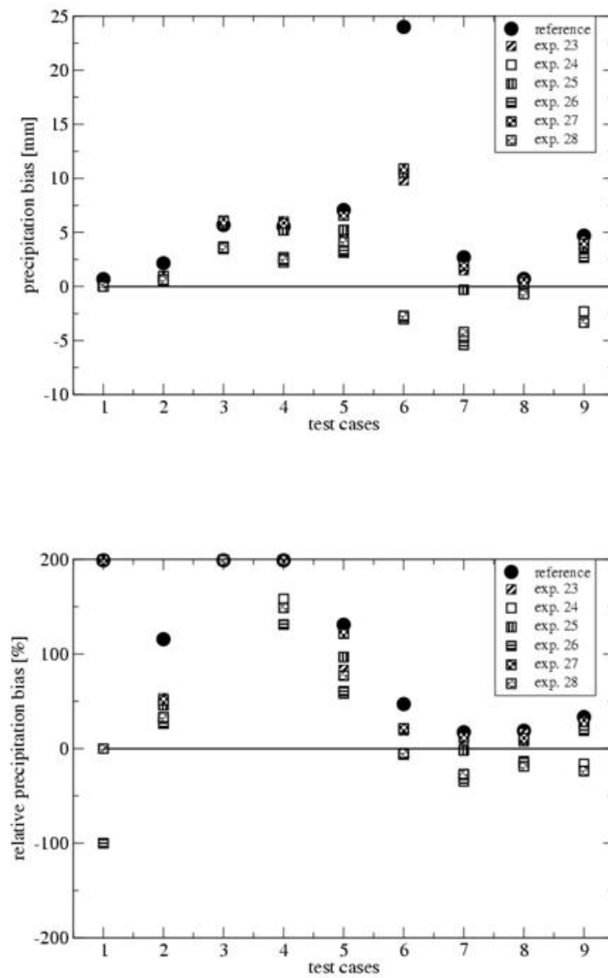
Figure 9: Absolute (upper panel) and relative (lower panel) precipitation bias ( (P_{exp} - P_{obs}) and (P_{exp} - P_{obs})/P_{obs} , respectively) of the reference simulation (black circles) and the cross experiments compared to the observations for cases with overestimation of stratiform precipitation. The test cases are 1, 2, 5, 6, 8, 10, 21, 22, and 24.
