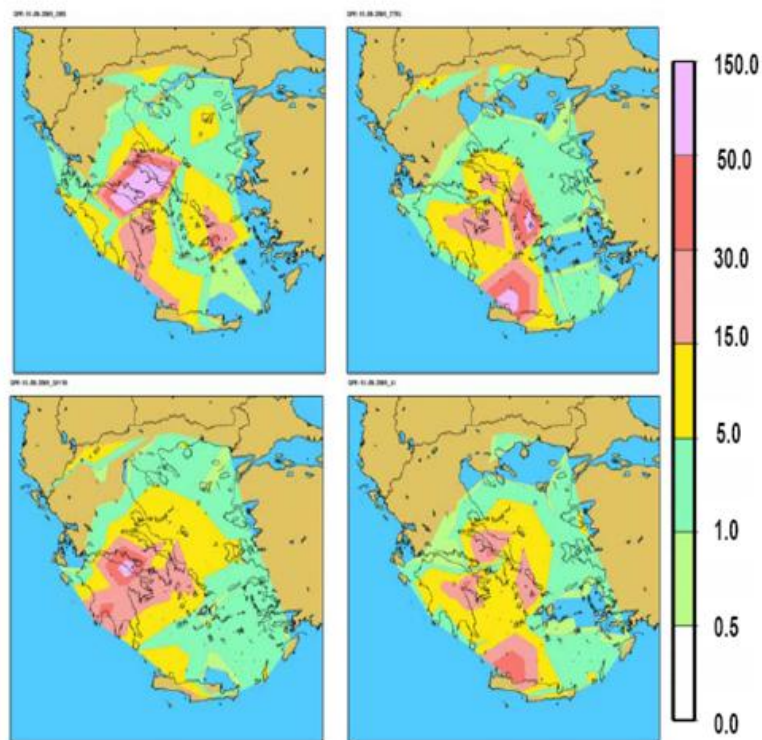
Figure 29: 24h precipitation sum in from 15.09.2005, 06 UTC - 16.09.2005, 06 UTC in the isohyet graphs based on synoptic observations from 63 meteorological stations (upper panel, left), in the reference simulation (upper panel right), in the sensitivity study with increase of water vapor mixing ratio (exp. 4, lower panel, left) and in the control experiment with COSMO 4.0 (exp. 23, lower panel, right).
