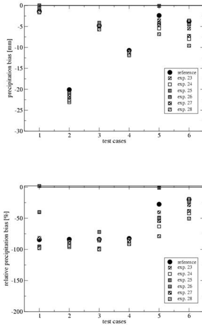
Figure 10: Absolute (upper panel) and relative (lower panel) precipitation bias ( (P_{exp} - P_{obs}) and (P_{exp} - P_{obs})/P_{obs} , respectively) of the reference simulation (black circles) and the cross experiments compared to the observations for cases with underestimation of convective precipitation. The test cases are 4, 9, 12, 15, 16, and 17.
