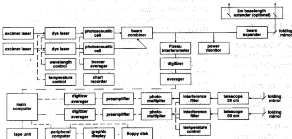
Abb. 2: Gesamtsystem Differential-Absorption-Lidar.
